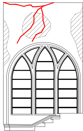
Elevation No 1 Datum Line : 57.00m
