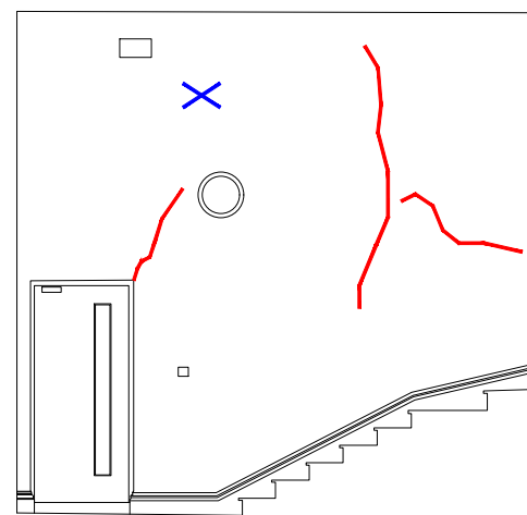
Elevation No 2 Datum Line : 57.00m
