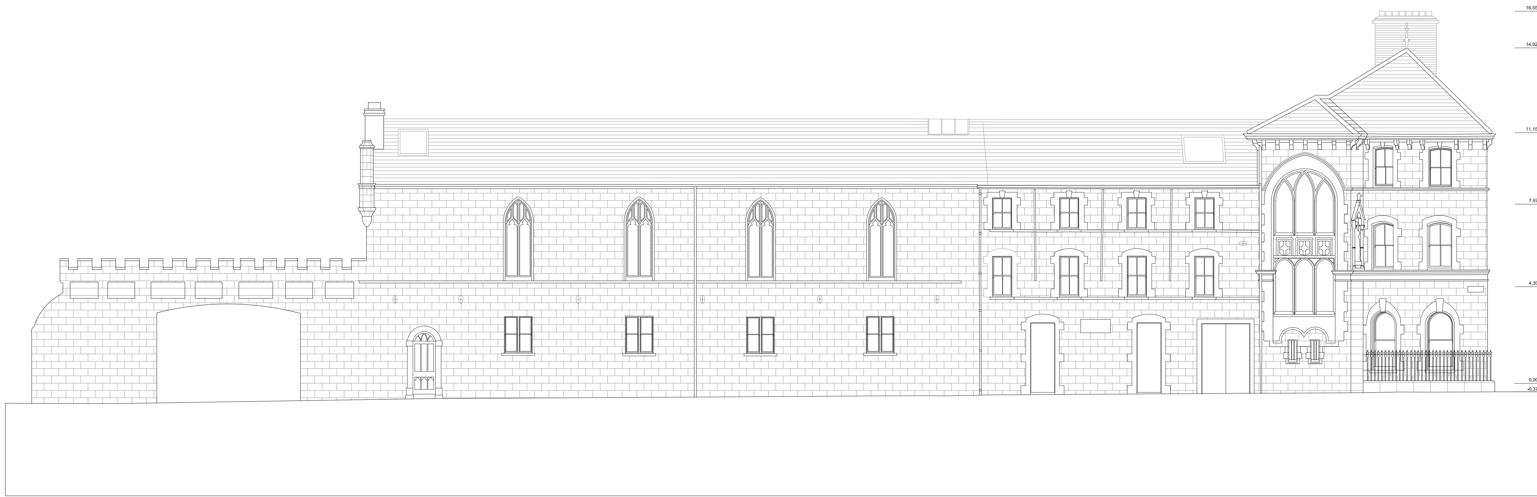
1 113 EXISTING WEST ELEVATION 1:100
