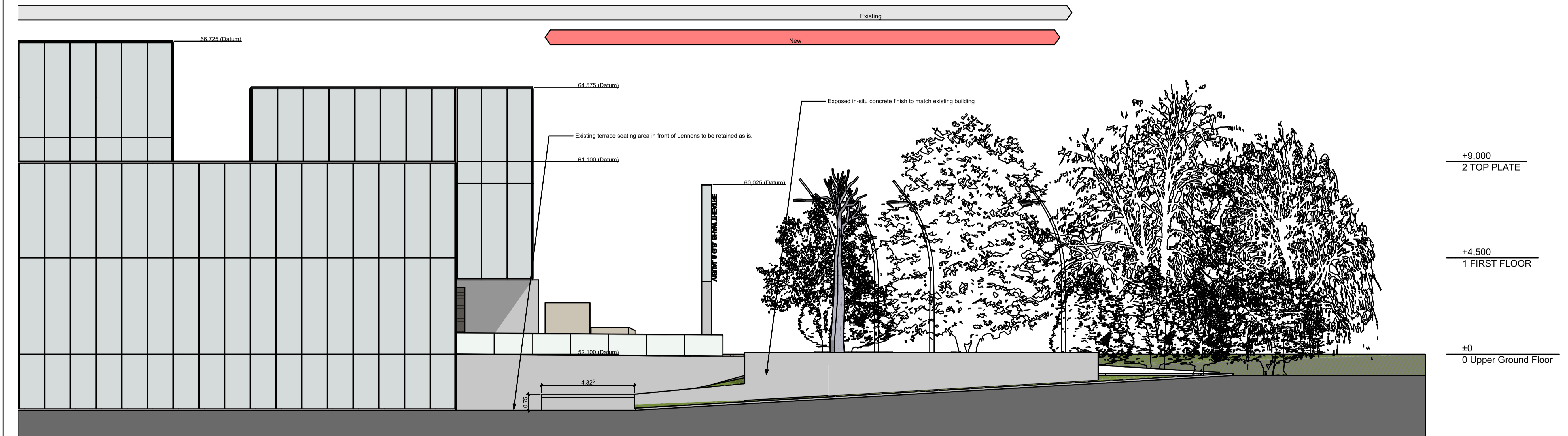
West Facing Elevation - Proposed 1:100
