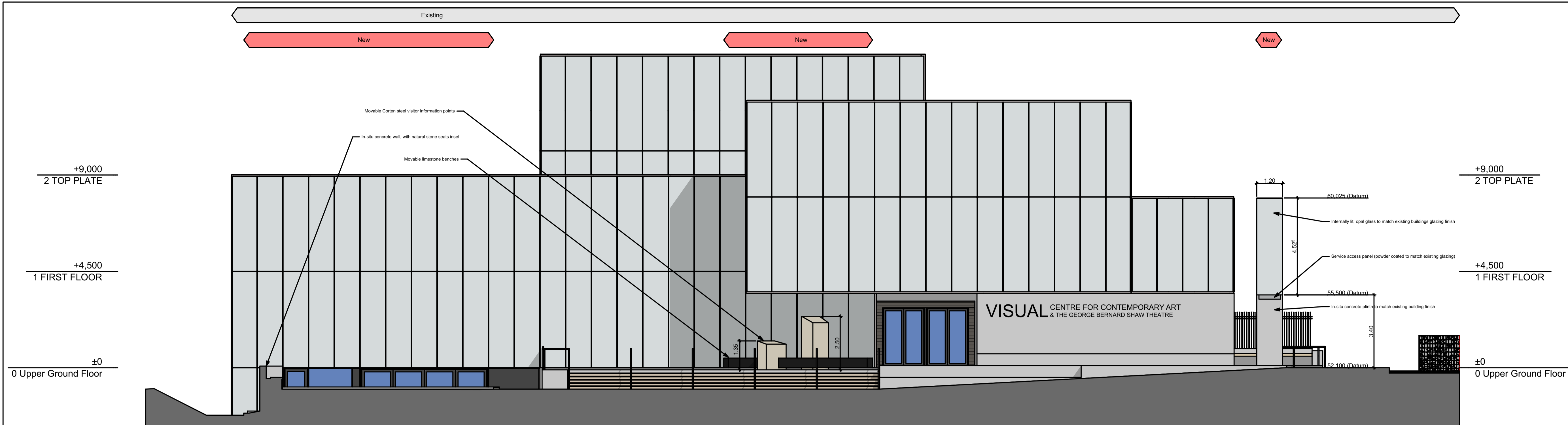
South Facing Elevation - Proposed 1:100
