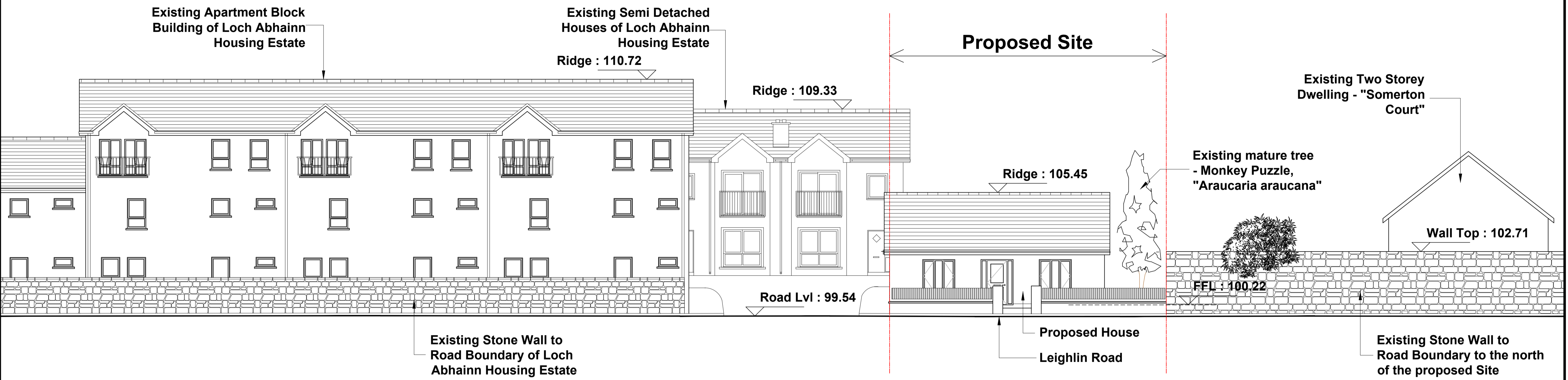
VIEW A-A - Streetscape Elevation SCALE 1:100
