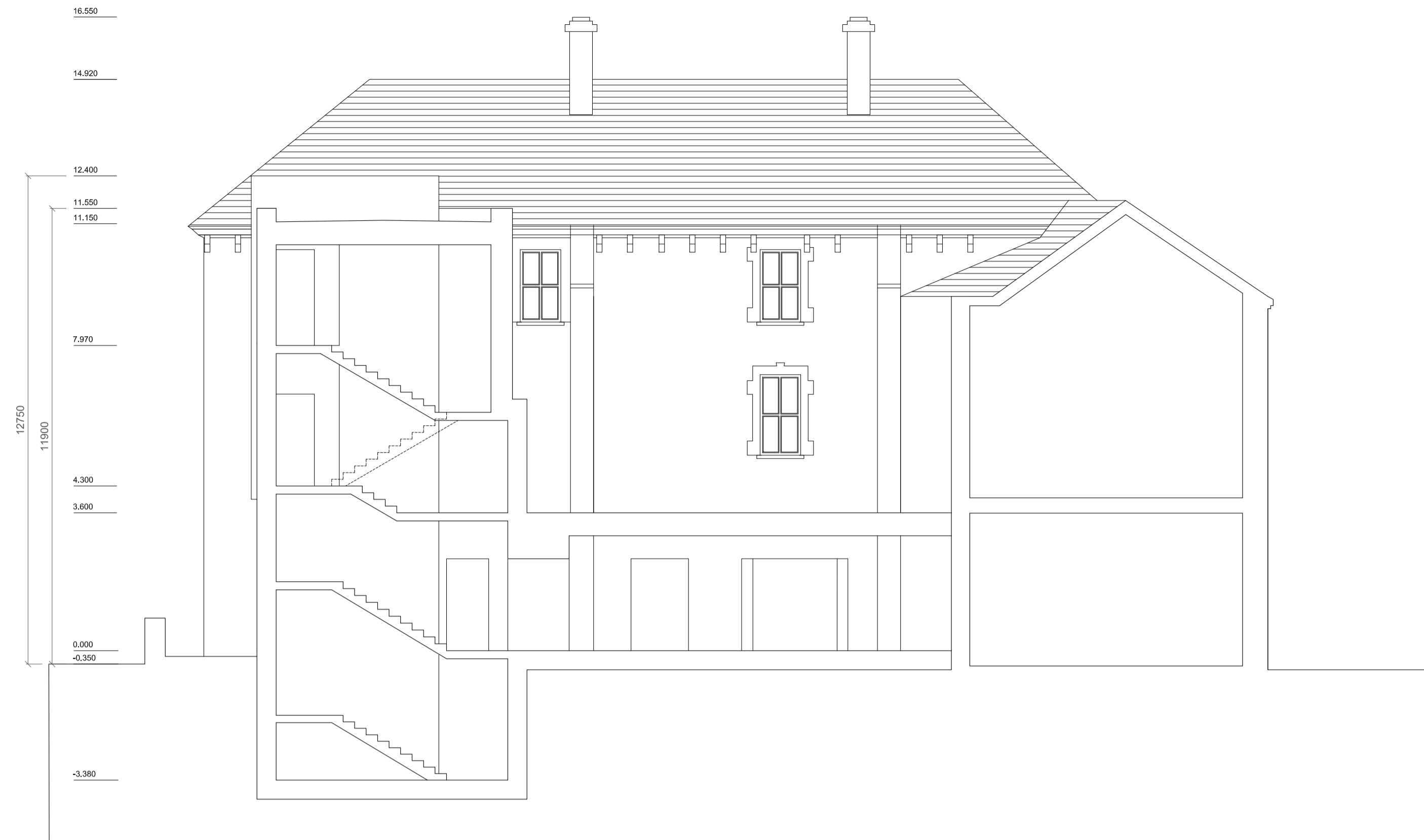
1 133 PROPOSED SECTION E-E 1:100
