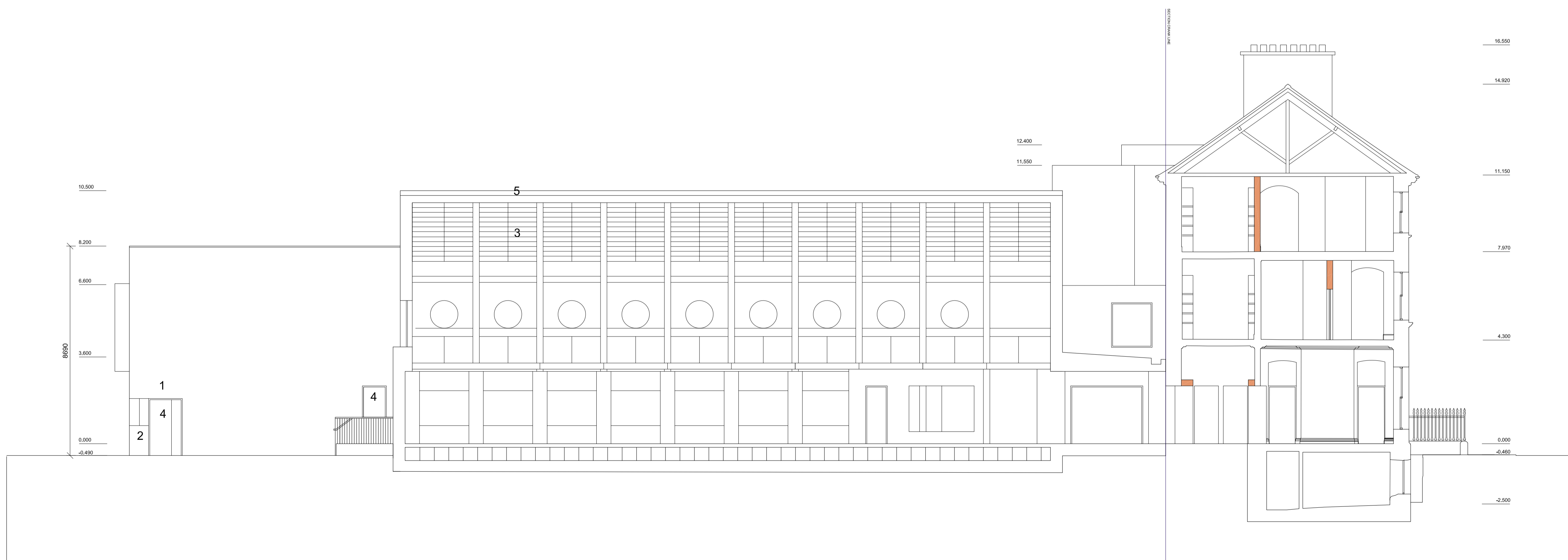
2 PROPOSED SECTION D-D 1:100
