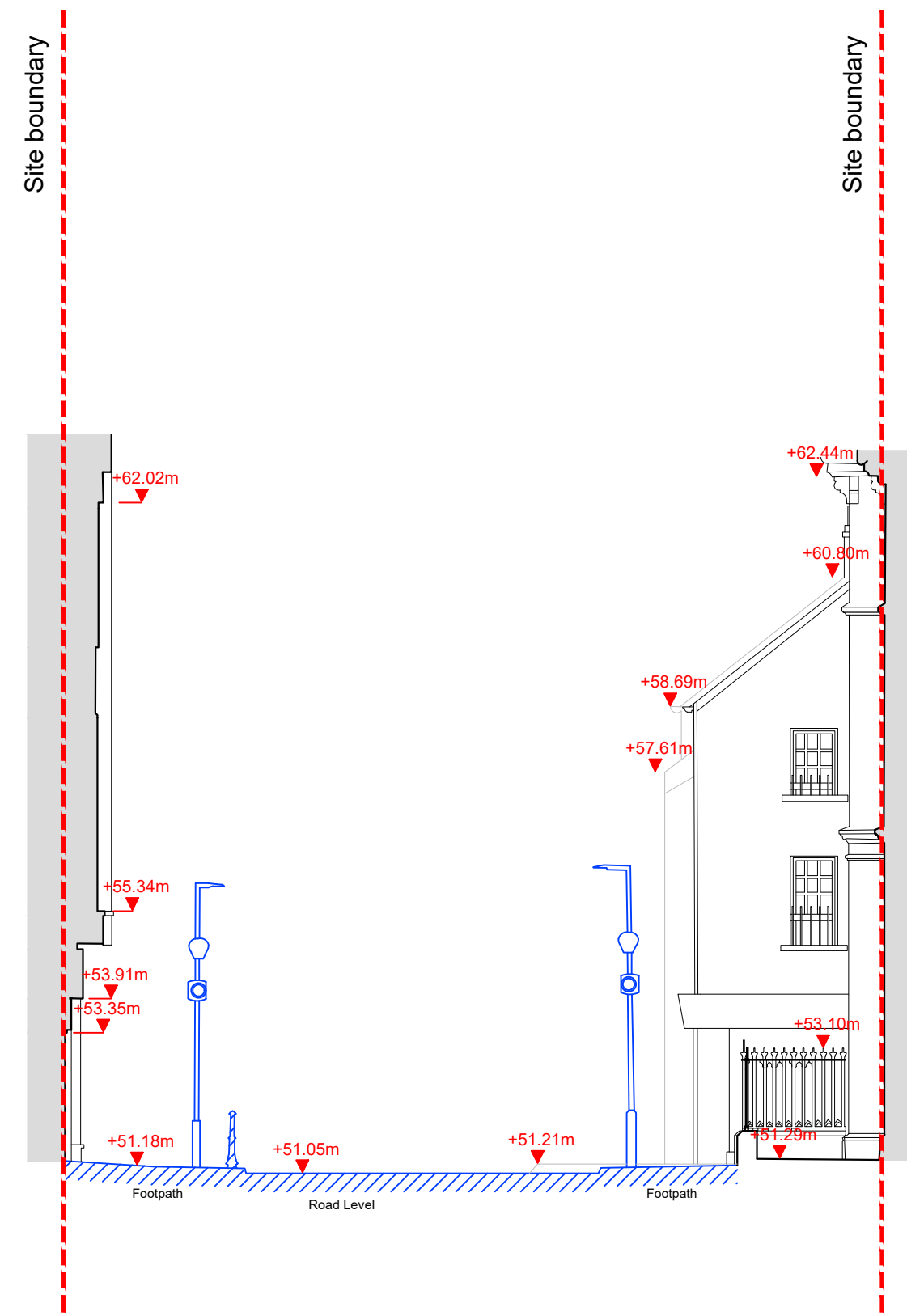
1 EXISTING SECTIONAL ELEVATION C-C 1:100 @ A1
